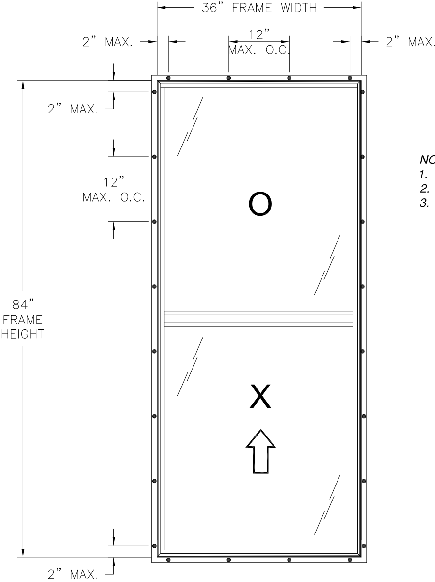
400/475 VINYL SINGLE HUNG WINDOW EXTERIOR VIEW
