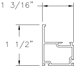
SASH STILE (4005) EXTRUDED RIGID PVC
