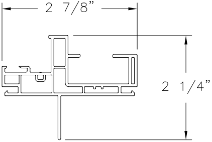
HEAD/JAMB (4000) EXTRUDED RIGID PVC
