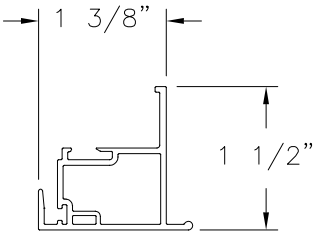
LOCK RAIL (4007) EXTRUDED RIGID PVC
