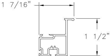
LIFT RAIL (4006) EXTRUDED RIGID PVC
