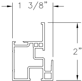
MEETING RAIL (4004) EXTRUDED RIGID PVC
