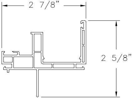
SILL (4002) EXTRUDED RIGID PVC
